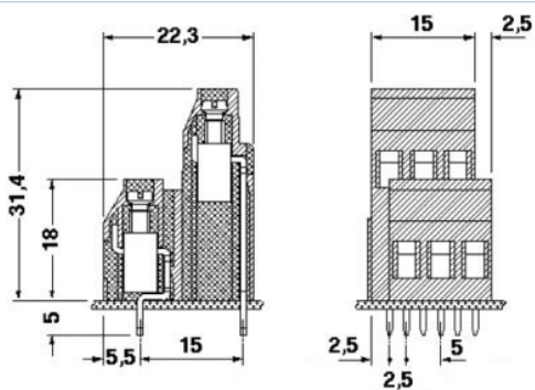
Dimensioned drawing
